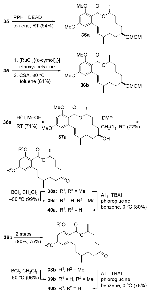
Scheme 5. Lactonization of hydroxy acid 35 and refunctionalization of lactones 36a and 36b . DMP = Dess–Martin periodinane, TBAI = tetrabutylammonium iodide.
