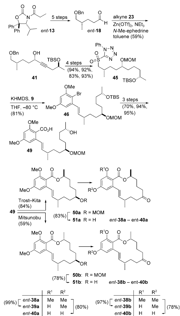
Scheme 6. Synthesis of the enantiomeric series of lactones ent - 38 – ent - 40 from propionyloxazolidinone ent - 13 ; for procedures and yields in this series, see the Supporting Information.
