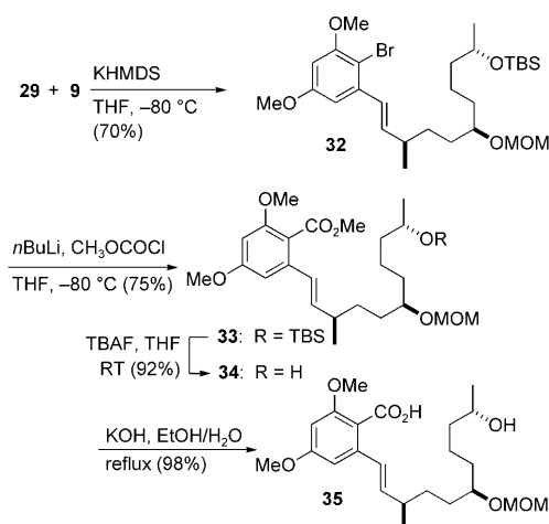
Scheme 4. Synthesis of seco acid 35 by means of Julia coupling and carboxylation. TBAF=tetrabutylammonium fluoride.
