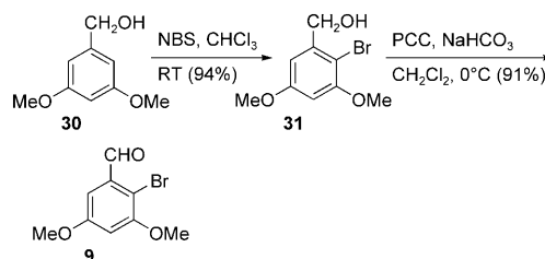
Scheme 3. Synthesis of 2-bromo-3,5-dimethoxybenzaldehyde ( 9 ). PCC=pyridinium chlorochromate.
