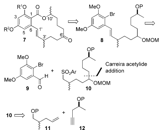
Scheme 1. Retrosynthetic analysis for zearalenone analogues of type 7 ; P=protecting group.
