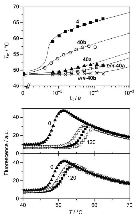
Figure 1. Hsp90N melting temperature ( T_m ) data as a function of added ligand concentration L_r . Panels on the bottom compare denaturation curves observed by fluorescence at 0 to 120 \mu M added ligand concentrations. The top of the bottom panels shows data for 40b , the lower panel for ent - 40a .
