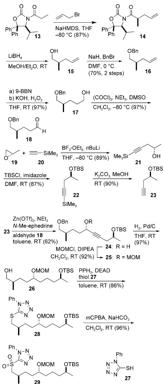
Scheme 2. Synthesis of aliphatic building block 29 . NaHMDS=sodium bis(trimethylsilyl)amide, Bn=benzyl, 9-BBN=9-borabicyclo[3.3.1]nonane, TBS=tert-butyldimethylsilyl, DIPEA= N,N -diisopropylethylamine, DEAD=diethyl azodicarboxylate, mCPBA= meta -chloroperoxybenzoic acid.
